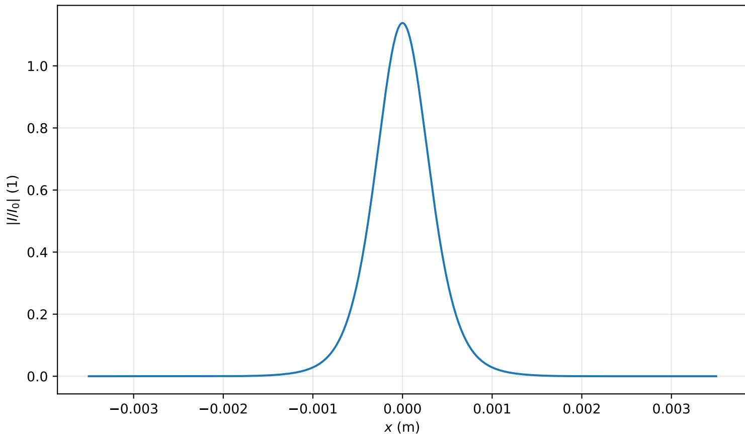
Intensity profile I(x, y = 0, z = 1.831m)/I_0 , \text{Pin}=0.7\text{Pcr} , artificial time
